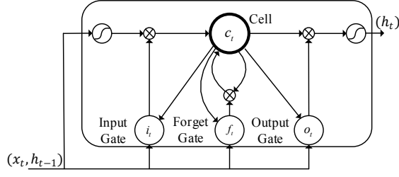
Fig. 3. Long short-term memory cell.
